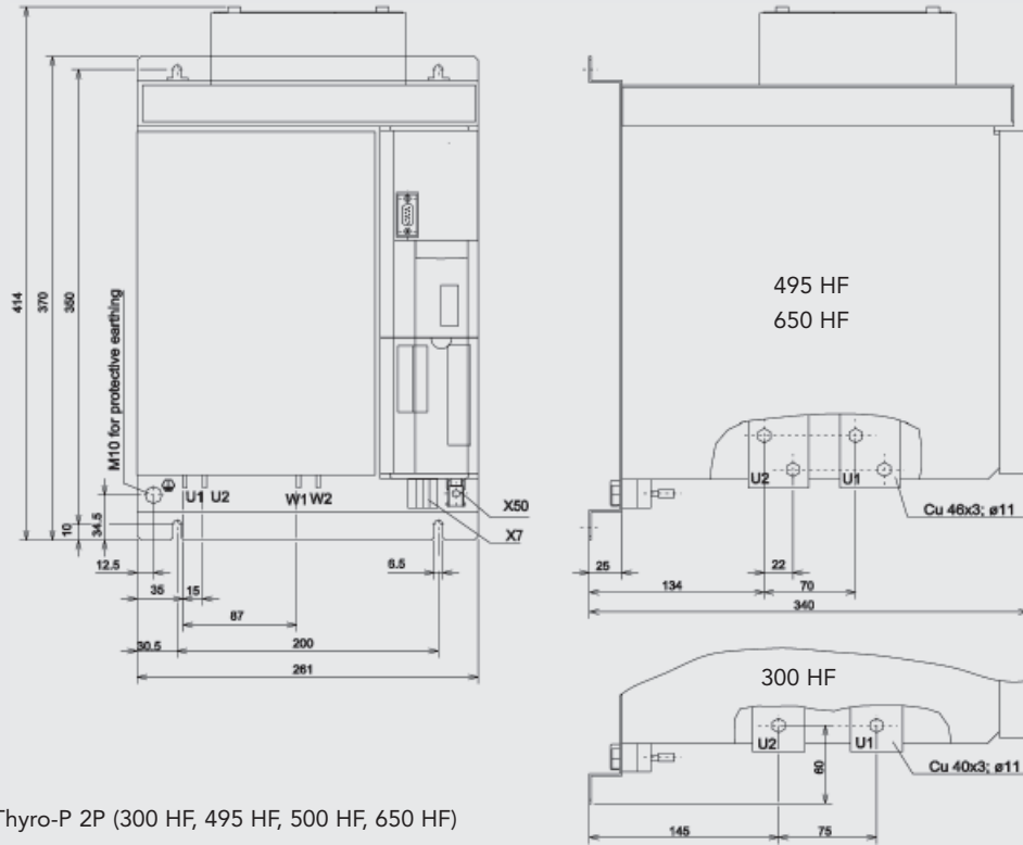
Dimensional Drawing 278
